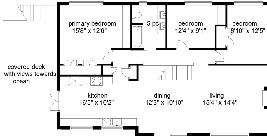
MAIN 1266 sq ft Ceiling height 8'0"
