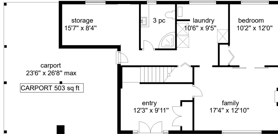
LOWER 956 sq ft Ceiling height 8'0"
